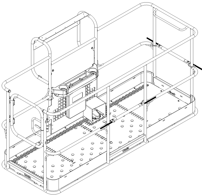
(1) Side Swing Gate Platform
